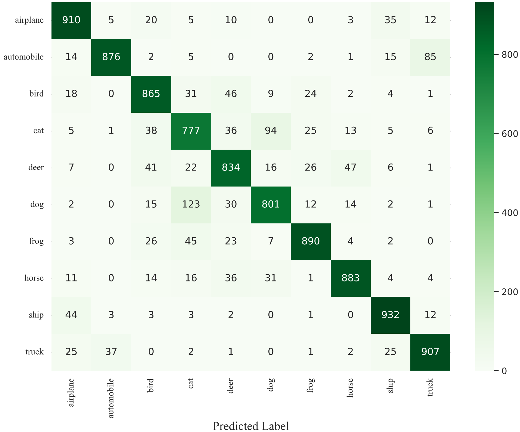
Confusion Matrix (ResNet50 Transfer Learning, Frozen Base)
